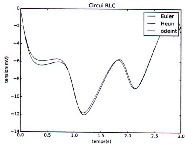
FIGURE 1: circuit RLC
